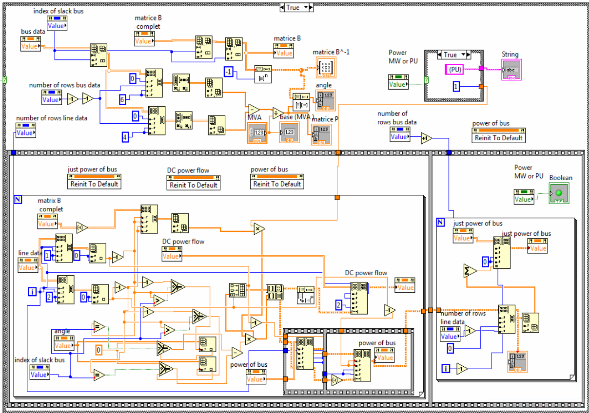
Fig. 2: Graphical program of DC load flow VI using LabVIEW.
