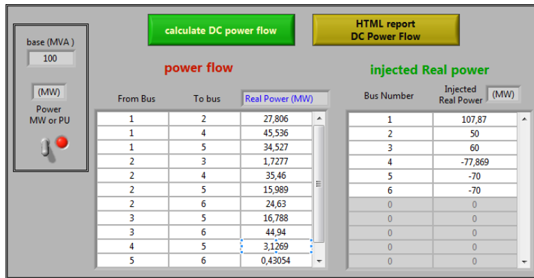
Fig. 5: DC power flow results by increasing the real power of load at bus 4 by AC losses.
